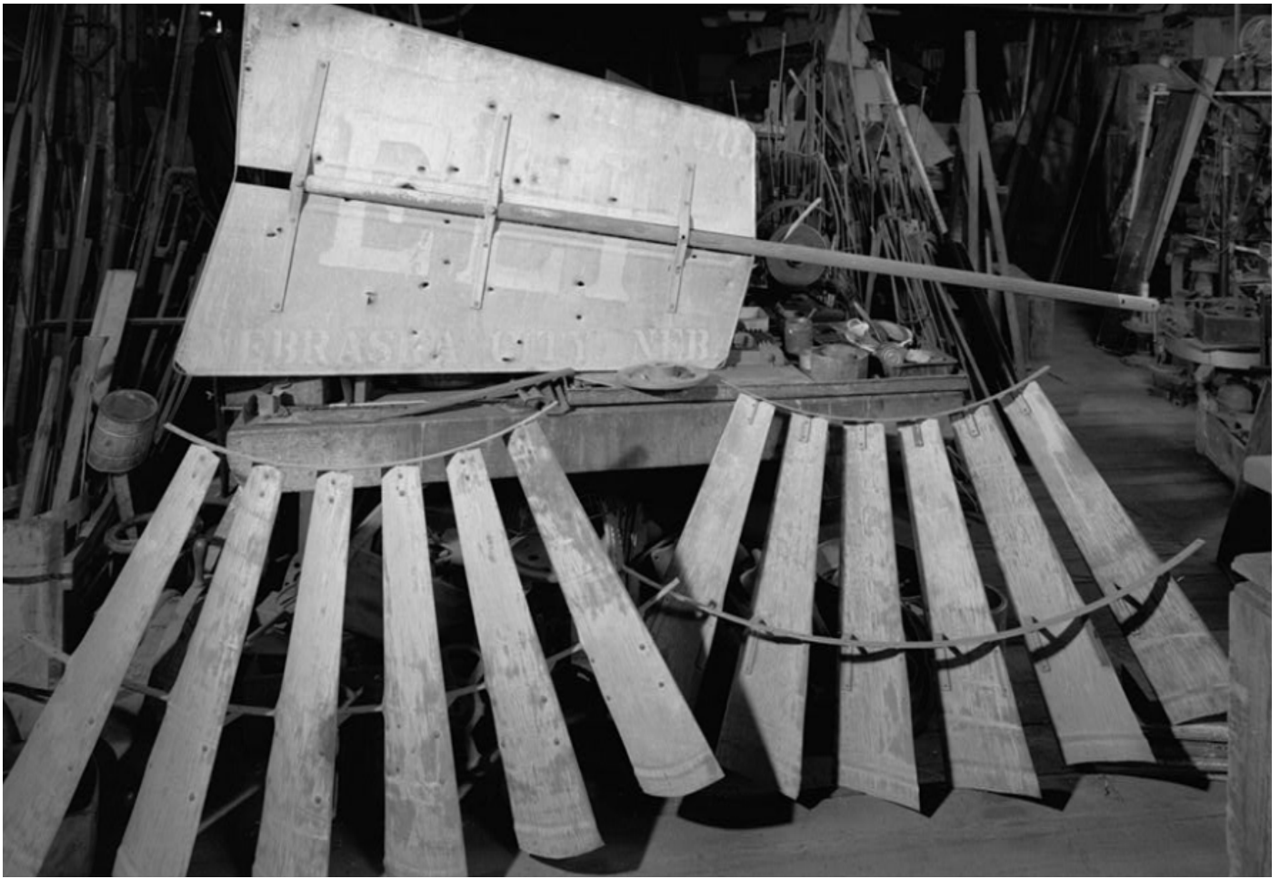
Windmill vane and blade assembly inside the Kregel Windmill Company Factory, a National Historic Landmark (photo by Jet Lowe, HAER)
